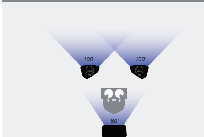
Small Club: 2 x P12 with 'PS Horn' for FOH, 1 x PS12 with standard horn for monitor
