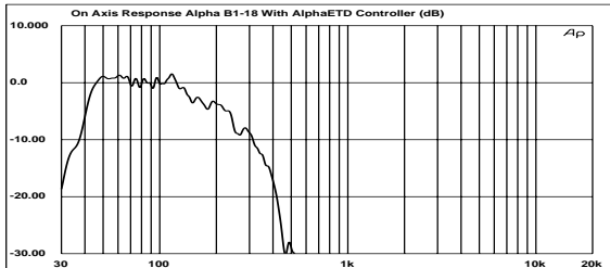
• Figure 3: Frequency Response with AlphaE TDcontroller (dB)
