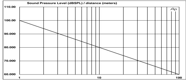
• Single Cabinet SPL versus Distance
