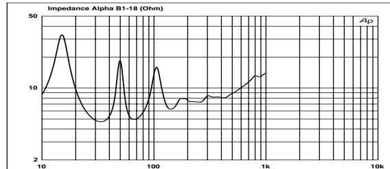
• Figure 4: Impedance (Ohms)
