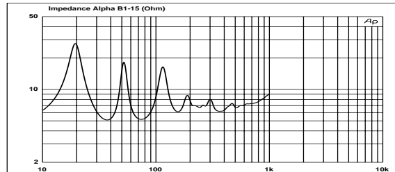
• Figure 6: Impedance (Ohms)
