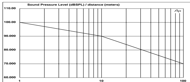
• Transition from cylindrical to spherical wave front
